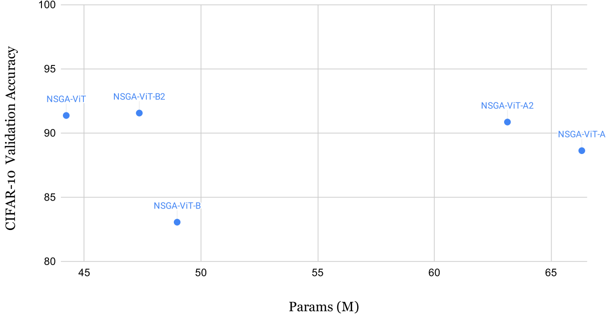
NSGA-ViT Comparison: Accuracy and Params
