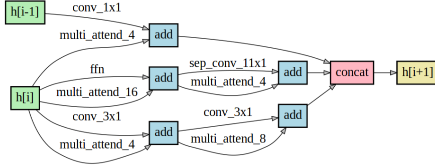
(c) NSGA-ViT-B2
