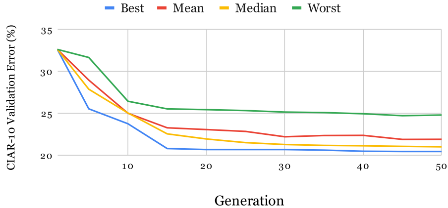
(b) CIFAR-10 validation error for Warm-Start setting.
