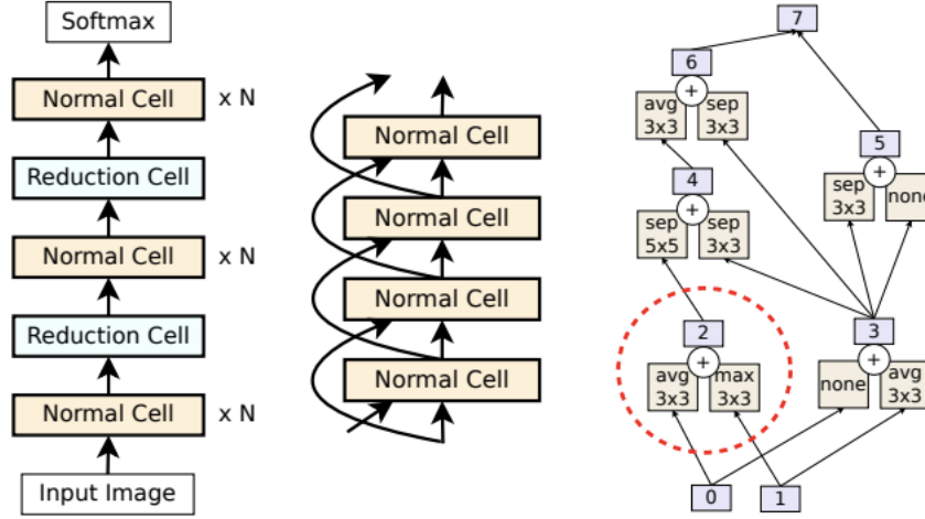
Figure 2.4: Illustration of Macro-level architecture from Zoph and Real [5, 6]. LEFT: the overall structure of the architecture trained on CIFAR-10. Normal cells are alternated with reduction cells (Not used in present study) at two depths in the network. Cells are stacked linearly. MIDDLE: the structure of the normal blocks in the model. Normal cells contain residual connections, allowing each cell to receive input from two cells before it. RIGHT: illustration of a possible cell from NAS-Net search space. The red circle highlights one operational block, made up of two operations from hidden states 0 and 1, respectively, combined by an addition operator. This cell contains 5 blocks with a final combiner.
