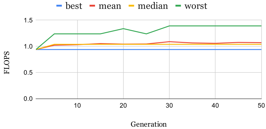
(b) Complexity metrics for the warm-start search
