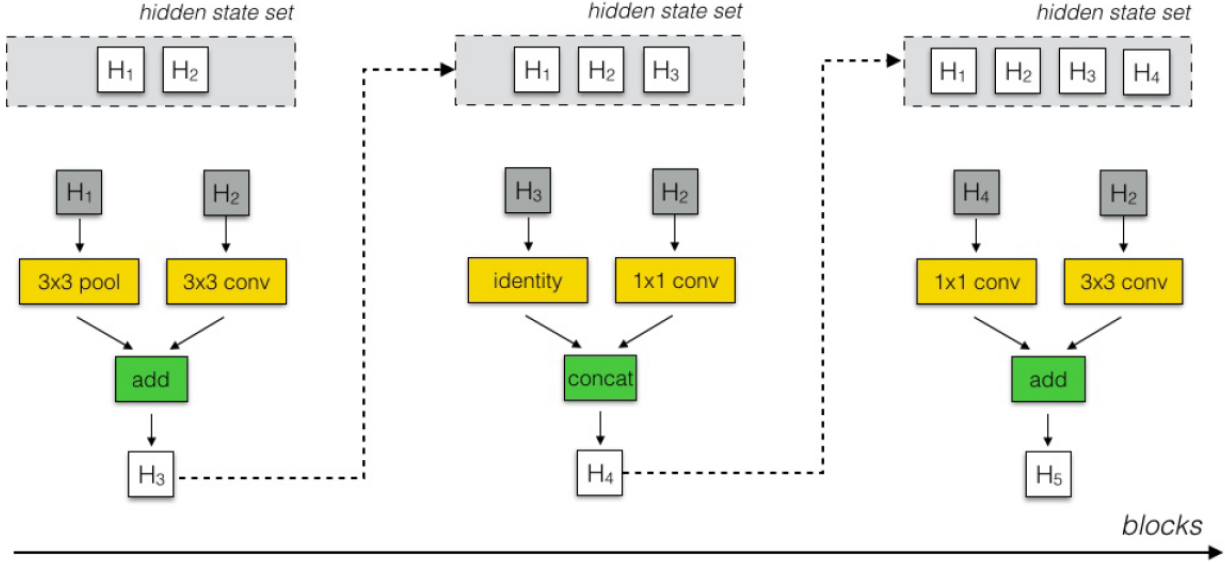
Figure 2.5: NAS-Net Search Space from Zoph et. al [5] . Cells are formed via a series of operational blocks. Blocks are formed by selecting two input hidden states, an operation to be performed on each state, and a combination operation to produce the new hidden state.
