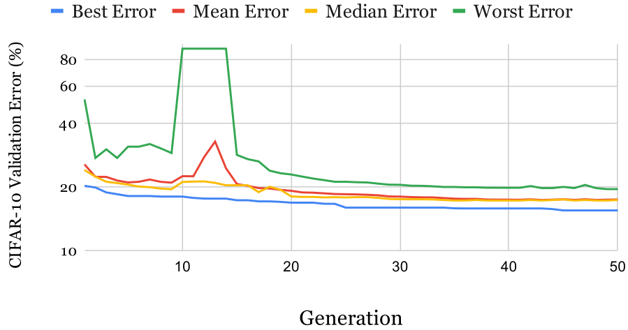
(a) CIFAR-10 validation error for Cold-Start setting.
