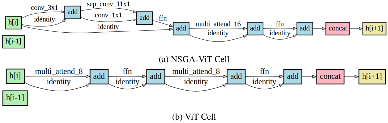
Figure 4.4: NSGA-ViT Architecture . TOP: NSGA-ViT architecture found in the search. BOTTOM: ViT architecture with 8-head MHSA layer. Each cell contains 2 transformer layers, resulting in 2 MHSA and FFN layers per cell.
