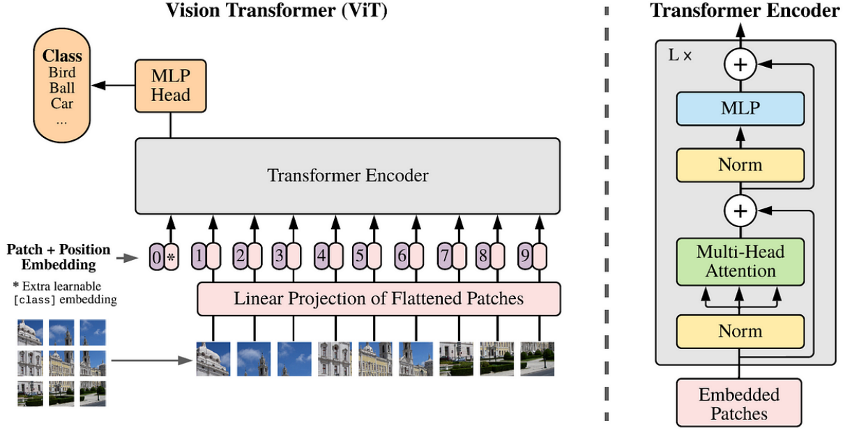
Figure 2.3: Vision transformer architecture from Dosovitskiy et. al [3]. Images are split into patches by an initial convolution layer before being flattened and adding position and class embedding. The resulting data is fed into a stack of transformer encoders, followed by an MLP classifier layer.
