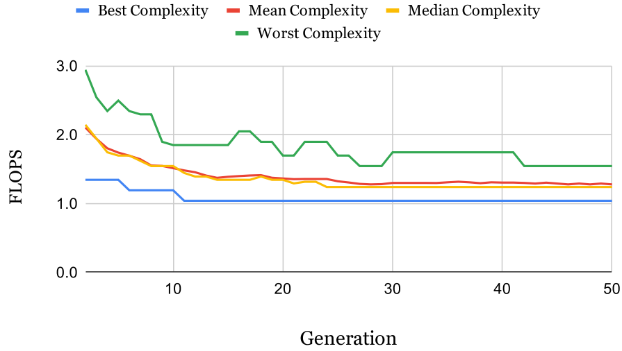
(a) Complexity metrics for the cold-start search
