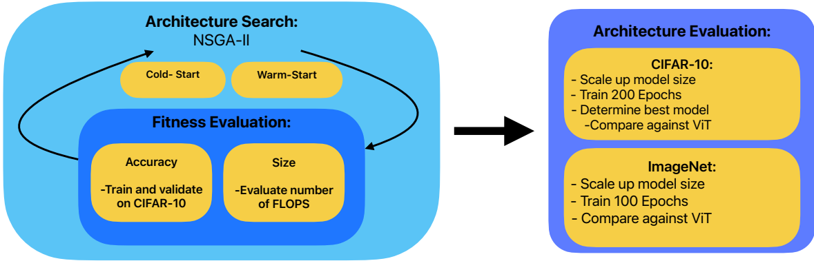
Figure 3.1: NSGA-ViT Procedure: NSGA-ViT is a two step procedure, consisting of architecture search and architecture evaluation. Architecture Search is bi-level optimization problem where architecture configurations are optimized in the outer layer, and connection weights are optimized via training in the inner layer. Architecture evaluation consists of training and evaluating discovered architectures against each other to determine the best solution, and then comparing against Transformers in the literature.
