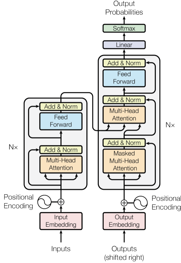
Figure 2.2: Transformer architecture from Vaswani 2017 [1] . Inputs are fed into the encoder layer, which uses multi-head self-attention followed by a feed forward layer. Labels (outputs) are fed into the decoder layer, as well as the output from the encoder. Finally, the decoder output is fed into a linear layer with a softmax classifier to produce the output probabilities.
