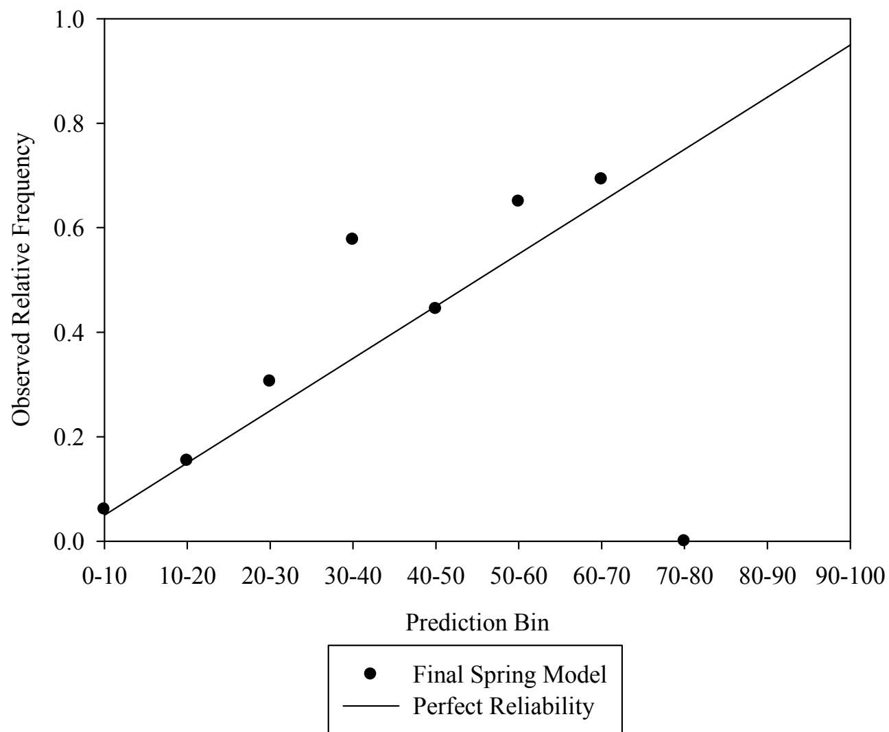
Figure 9: The reliability diagram for the final spring model, evaluation data set.
