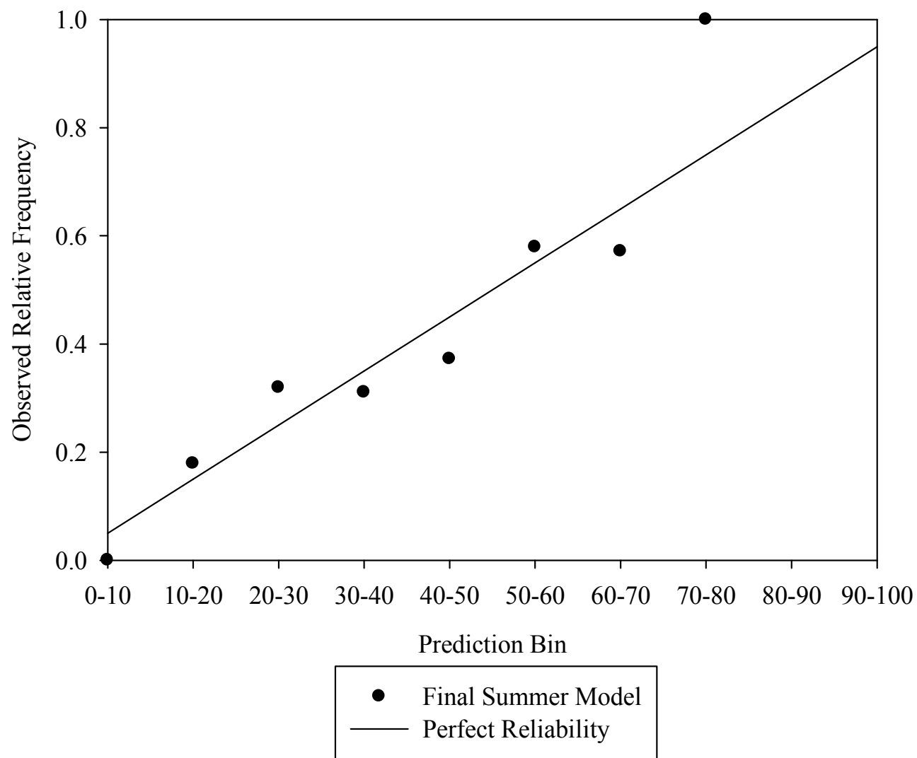
Figure 11: The reliability diagram for the final summer model, evaluation data set.
