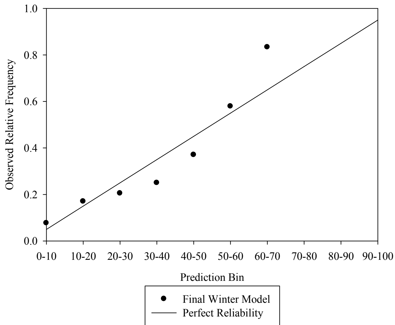
Figure 7: The reliability diagram for the final winter model, evaluation data set.
