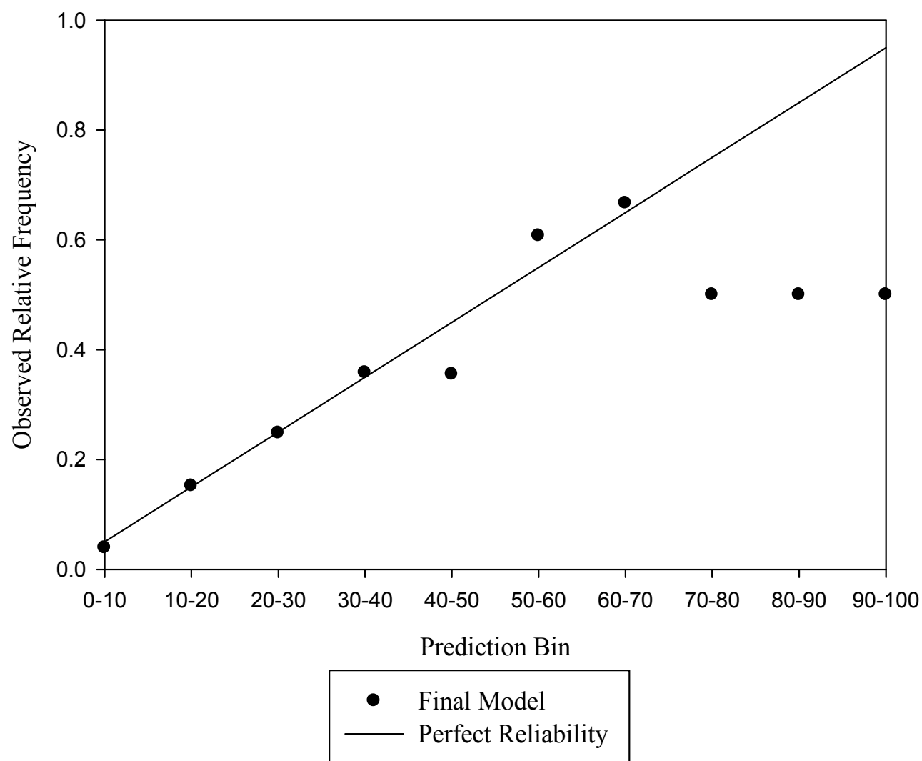
Figure 15: Reliability diagram for the final ensemble model, evaluation data set.
