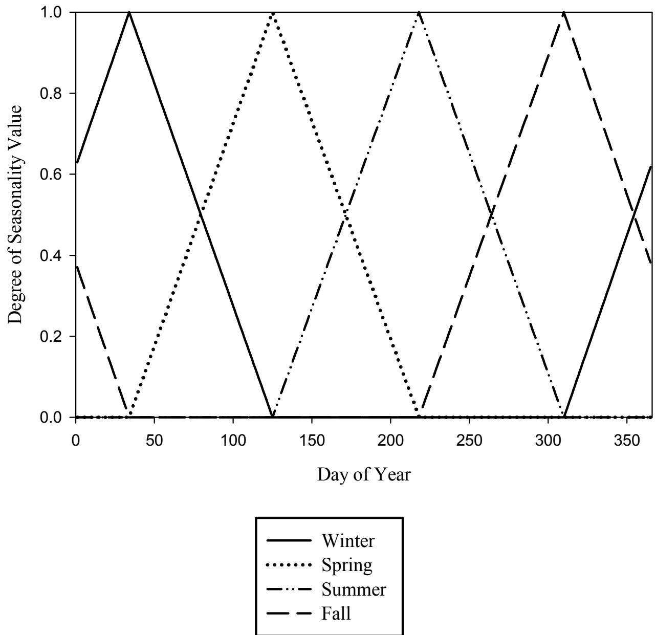
Figure 2: Inputs representing seasonal values of the four seasons, fuzzy logic type membership functions.
